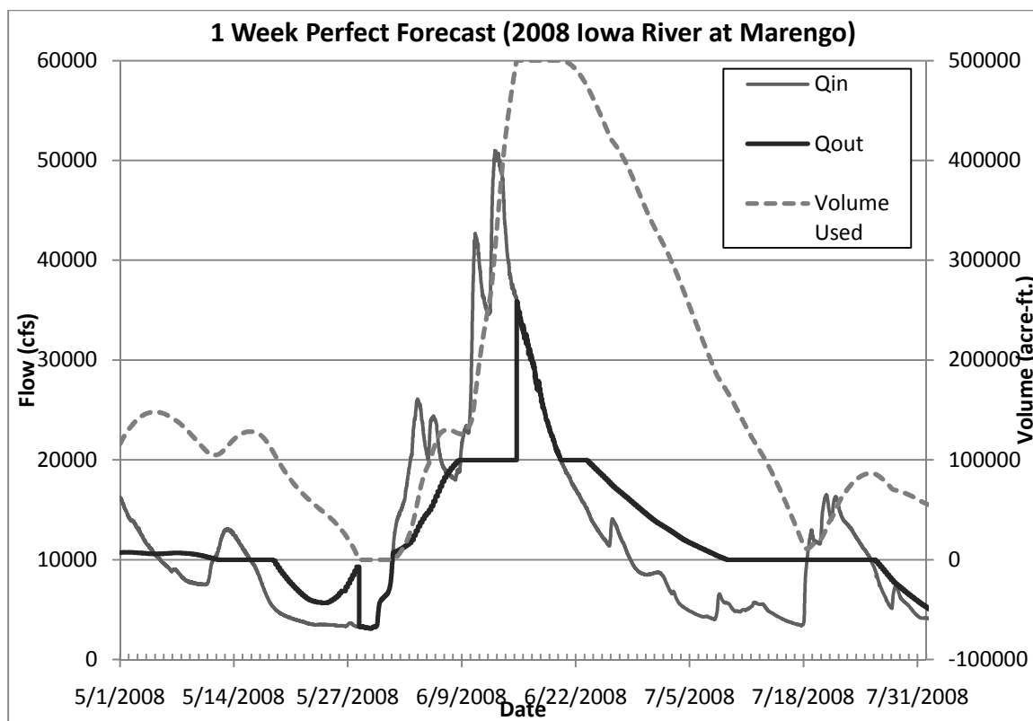
Figure 1-9: One week perfect forecast simulation for the 2008 Iowa River flood.
