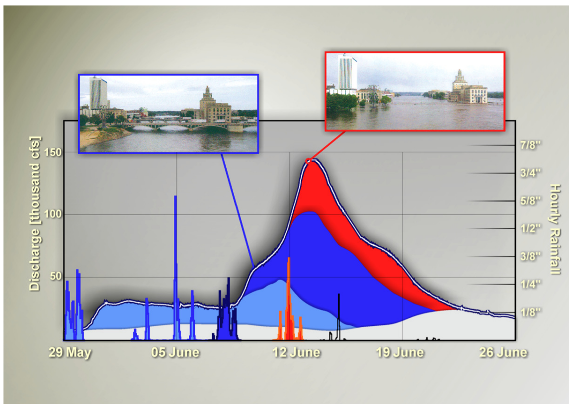
Figure 3-1: Figure showing the portion of the flood wave in Cedar Rapids caused by the rainfall events leading up to the flood.*
