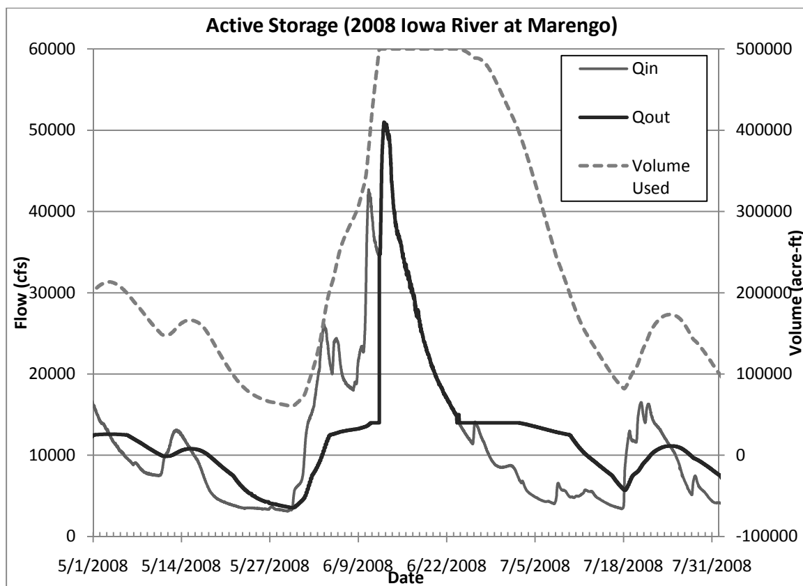
Figure 1-4: Active storage reservoir using the specified release rules for the 2008 Flood.
